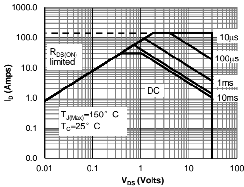
Figure 9: Maximum Forward Biased Safe Operating Area (Note F) V GS > or equal to 4.5V
